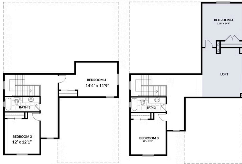
Second Floor • 9' Ceiling
